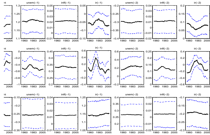
Figure 1: Time Varying Parameters (TV-VAR model)
