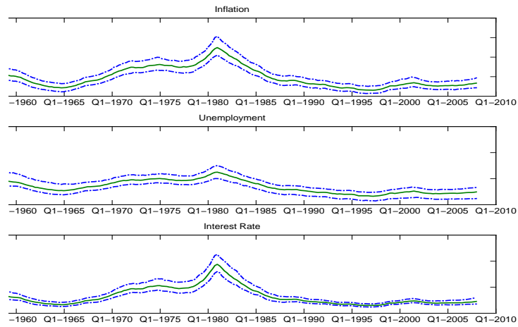
Figure 2: Time Varying Stochastic Volatility (TV-VAR model)
