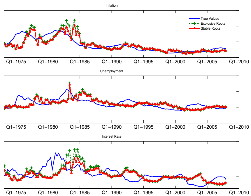
Figure 3: Three Years Ahead Forecast
